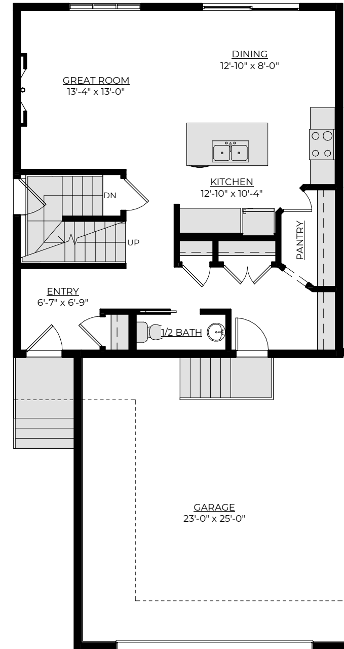
Main Floor Plan 783 ft 2
